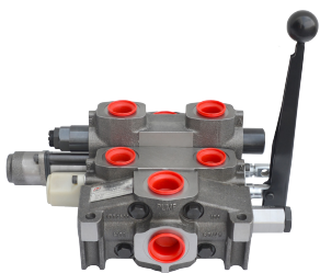
Hyd kickout with handle
