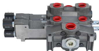
Solenoid control
