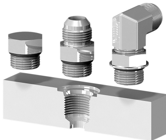
Straight Thread Port Assembly
